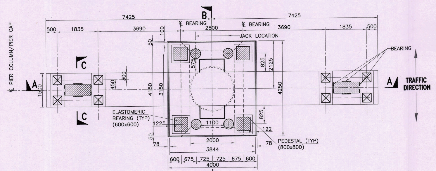
TOP PLAN OF PIER CAP (SHOWING PEDESTAL AND BEARING) (SCALE 1:100)
